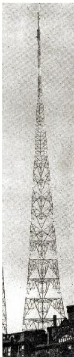
709' Free-Standing Tower erected on building for Station KRNT in Des Moines, Ia.
